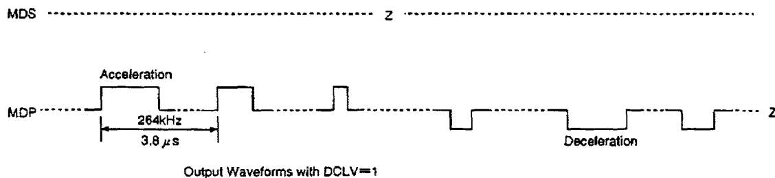
Timing Chart 1-16
