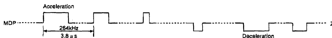
Timing Chart 1-18
