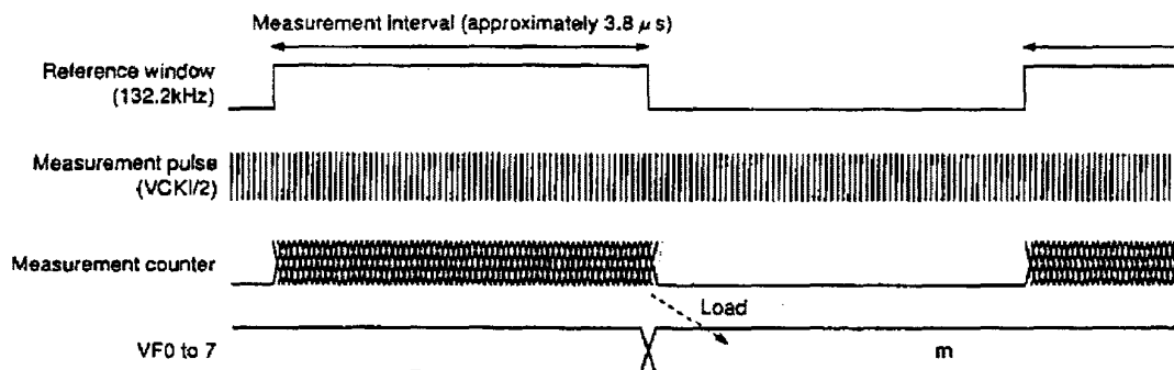
Timing Chart 2-5
