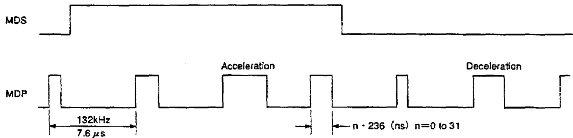
Timing Chart 1-14
