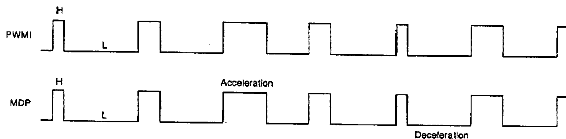
Timing Chart 1-20
