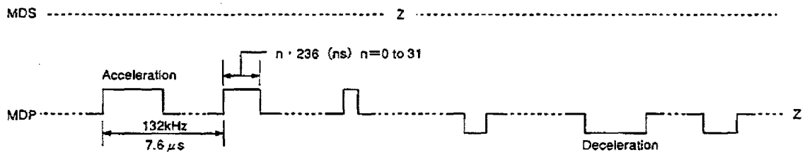
Timing Chart 1-14
