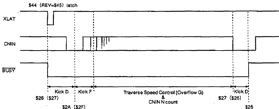
Fig. 4-12 (b). Fine Search Timing Chart
