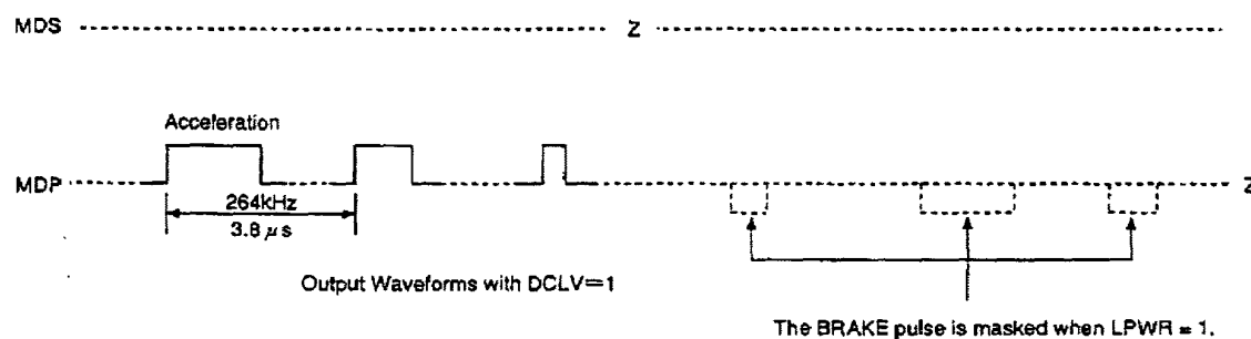
Timing Chart 1-17
