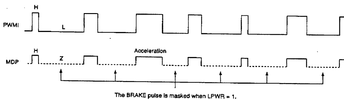
Timing Chart 1-20
