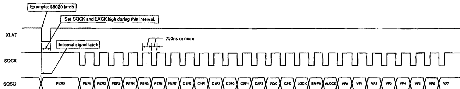
Timing Chart 2-4
