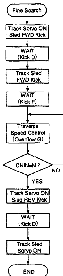
Fig. 4-12 (a). Fine Search Flow Chart
