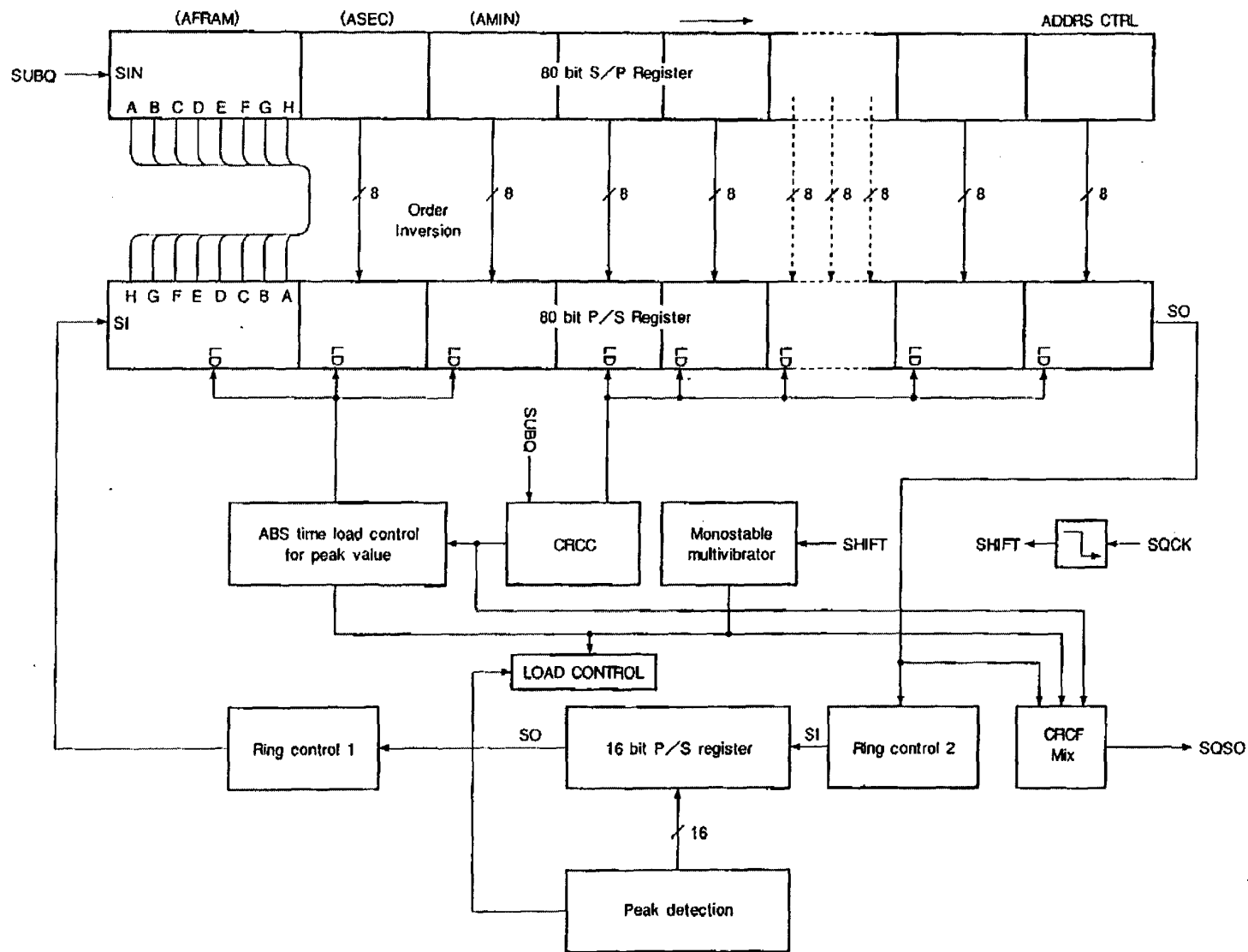
Block Diagram 2-2
