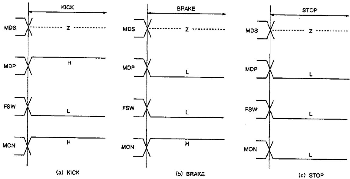
Timing Chart 1-7
