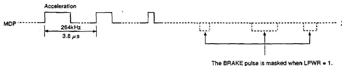
Timing Chart 1-18
