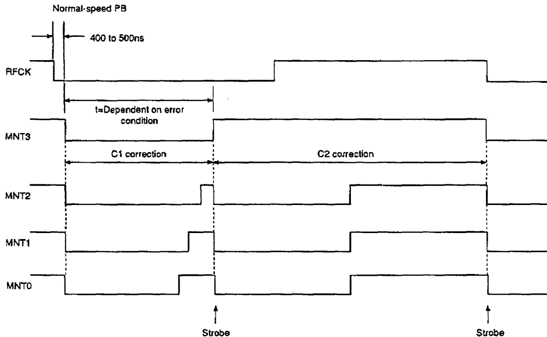
Timing Chart 4-3
