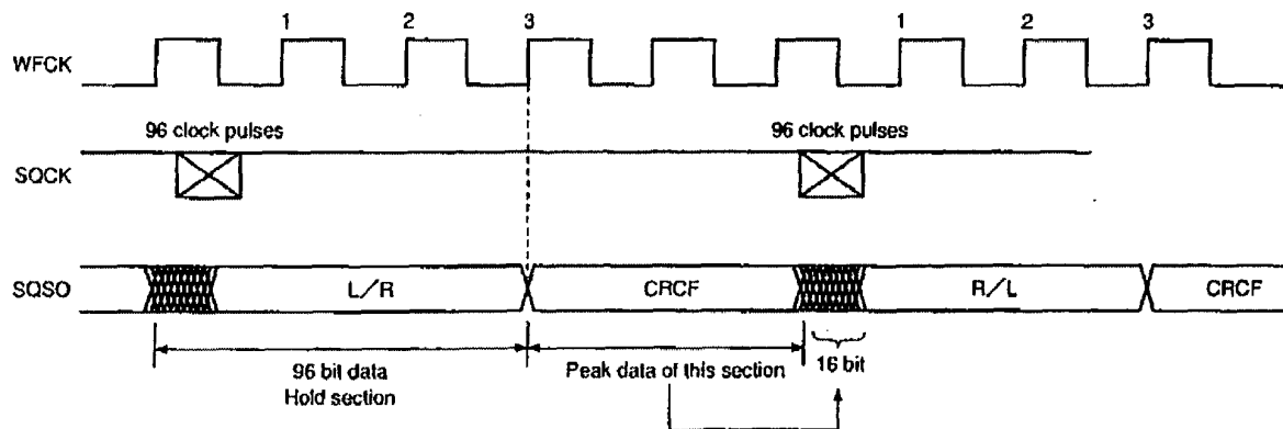
Level Meter Timing
