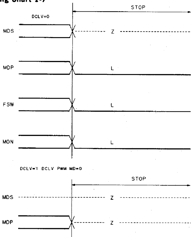
Timing Chart 1-7
