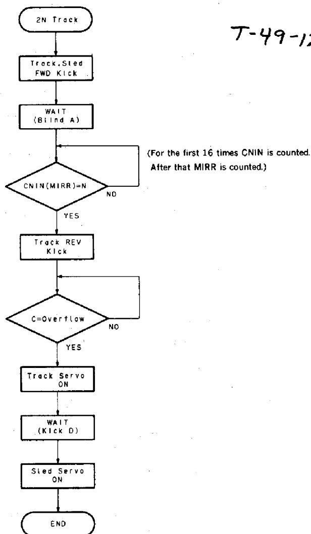
Figure 3-11 (a) Flowchart of 2N track jump
