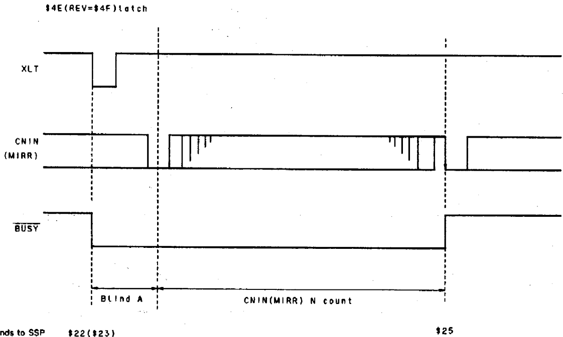
Figure 3-12 (b) Timing chart for N track move
