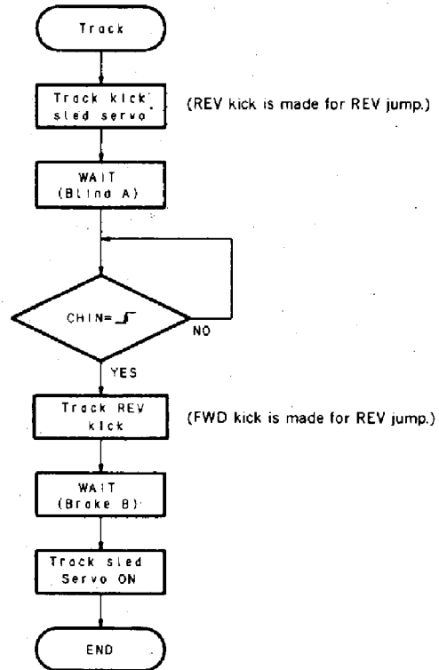
Figure 3-9 (a) Flowchart of 1-track jump
