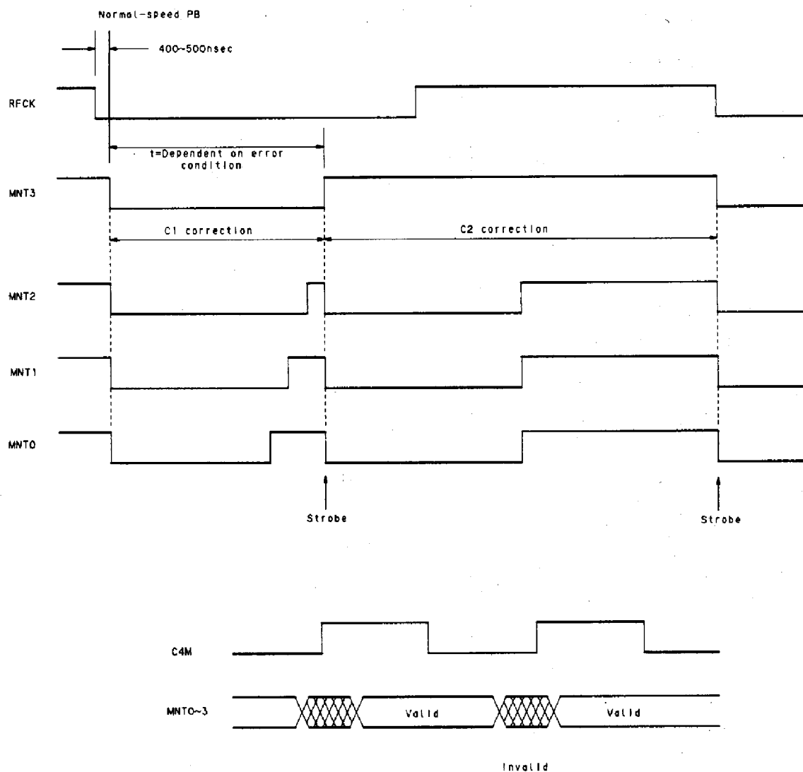
Timing Chart 3-3
