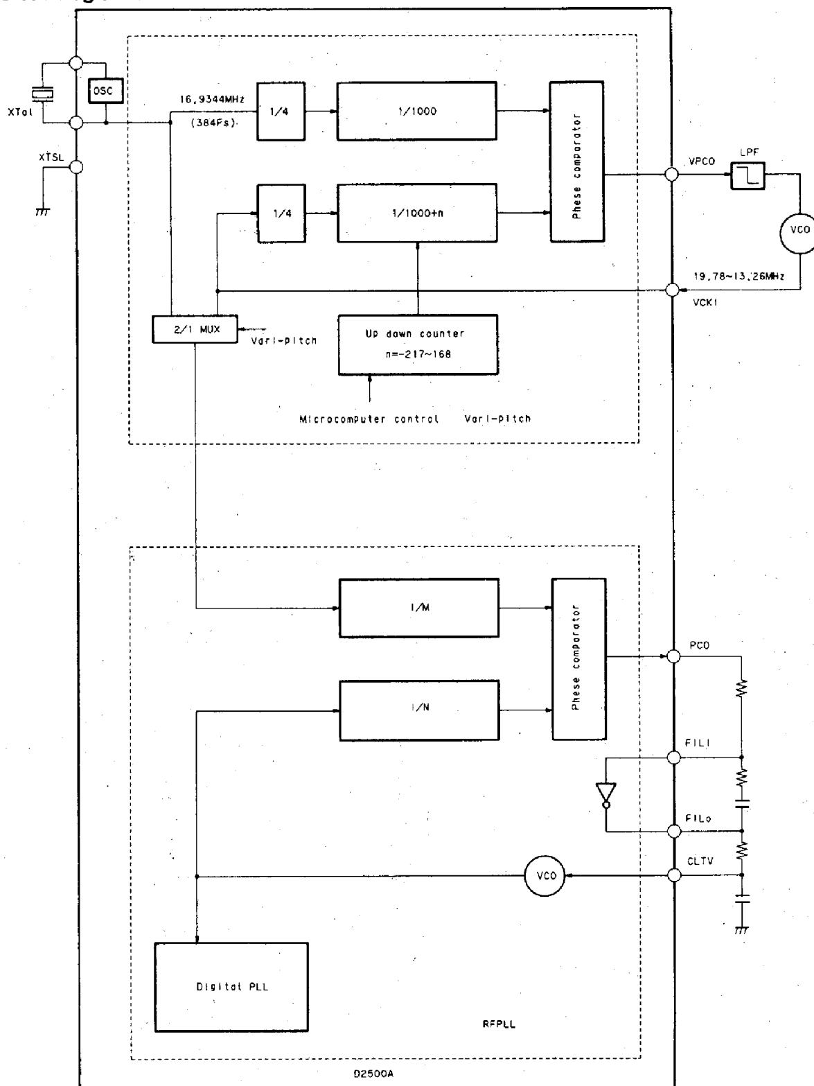
Block Diagram 3-1
