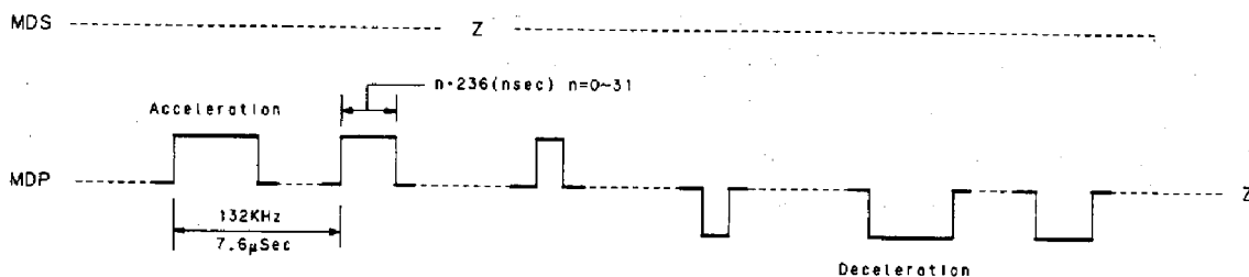
Timing Chart 1-6
