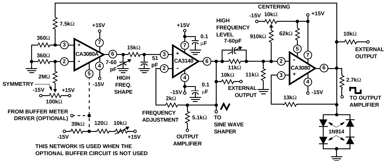
FIGURE 10A. CIRCUIT
